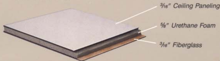
CEILING CUT-AWAY
